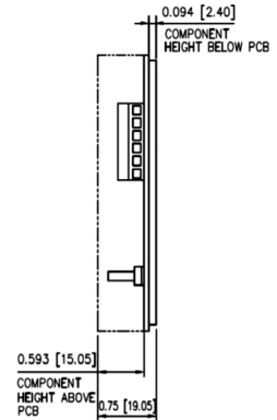
J4: PGPF Connector (5) (optional)
