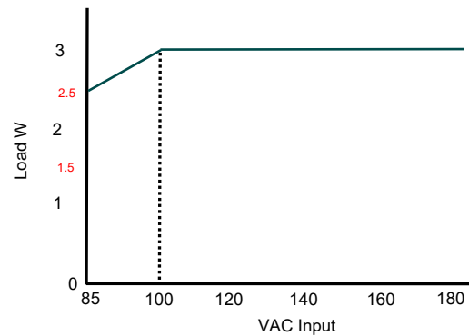
AC input curve
