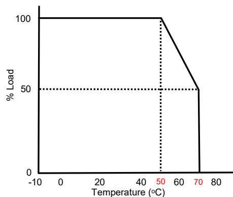
Derating curve
