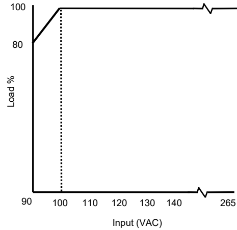
AC Input Derating Curve
