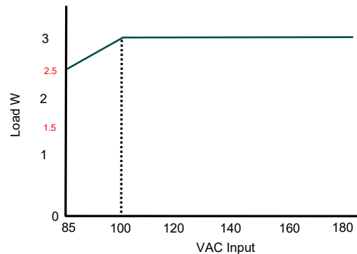
AC input curve
