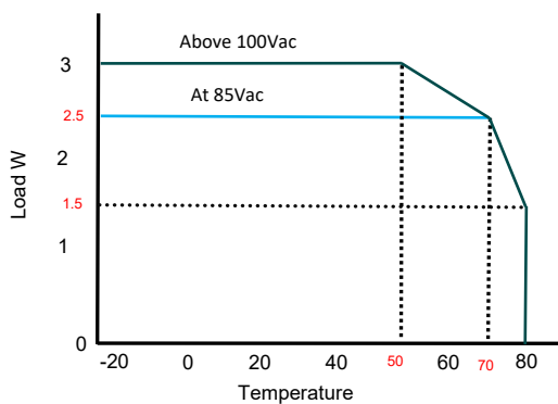
Derating curve 3.3V /5V
