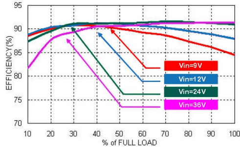
RED60-24S05W Efficiency vs. Output Load
