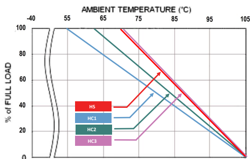
RED60-24S05 Derating curve with heatsink
