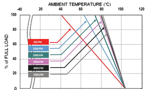
RED60-24S05 Derating curve
