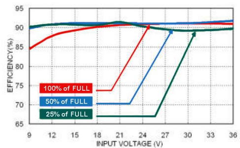
RED60-24S05W Efficiency vs. Input Voltage
