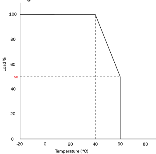
Derating curve
