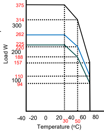
Power Derating Curve 15V
