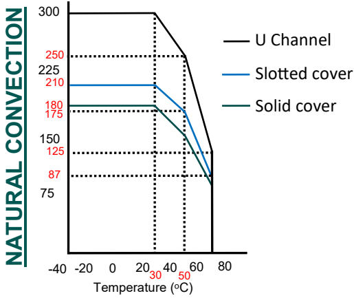
Power Derating Curve 12V
