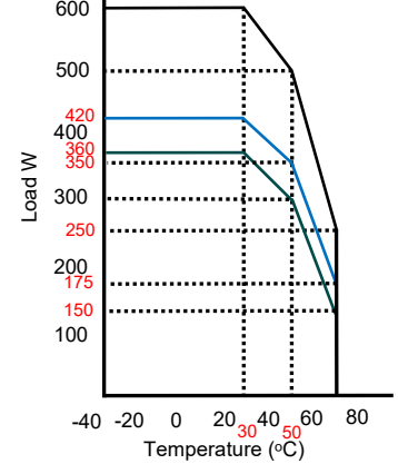
Power Derating Curve Others
