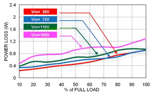
Power Dissipation Versus Output Load
