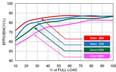
Efficiency Versus Output Load
