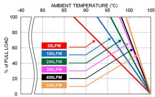
Derating Output Load Versus Ambient Temperature and Airflow Vin(nom)
