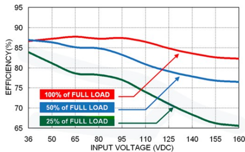
Efficiency Versus Input Voltage.
