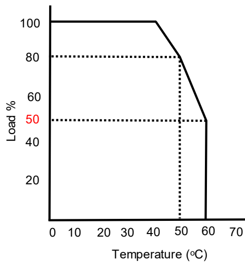
Derating curve
