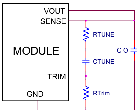
Figure 47. Circuit diagram showing connection of R_{TUNE} and C_{TUNE} to tune the control loop of the module.
