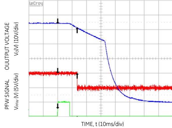
Figure 12. PFWS alarmed 19.6ms prior to Vo < 40V, output load: 38A, V IN = 185V AC .
