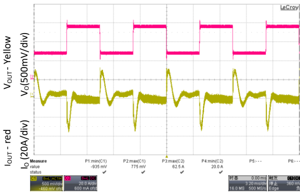
Figure 7. Transient response 65V DC load step 10 – 60%, Slew rate: 1A/ \mu s, V_{IN} = 230V AC
