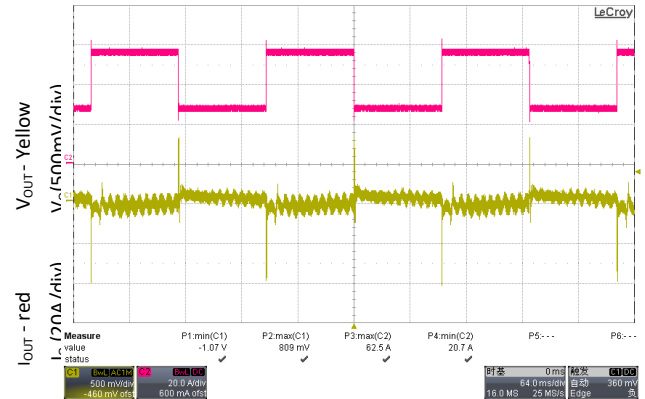
Figure 8. Transient response 65V DC load step 10 – 60%, Slew rate: 1A/ \mu s, V_{IN} = 230V AC
