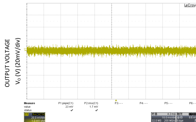
Figure 6. 5V DC output ripple and noise, all full load, V IN = 185V AC , 20MHz bandwidth
