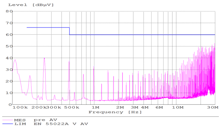
Figure 22. EMC Consideration
