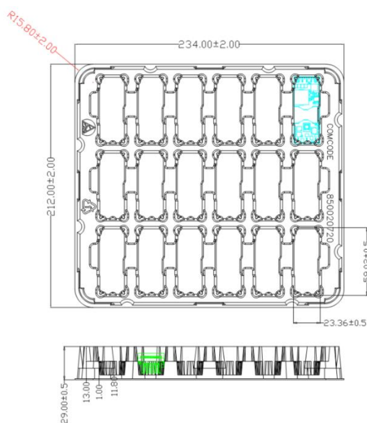
Open Frame Module Tray
