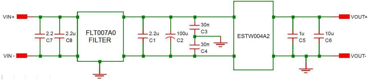
Figure 23. EMC Considerations
