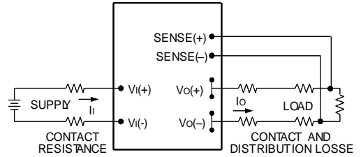
Figure 10. Circuit Configuration for remote sense .
