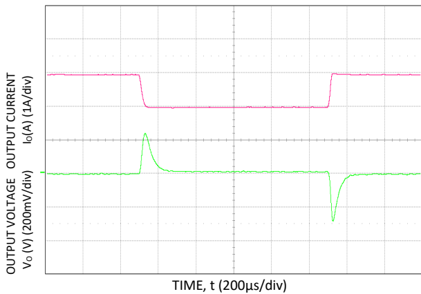
Figure 3. Transient Response to 0.1A/ \mu S Dynamic Load Change from 50% to 75% to 50% of full load, V_{IN}=48V .
