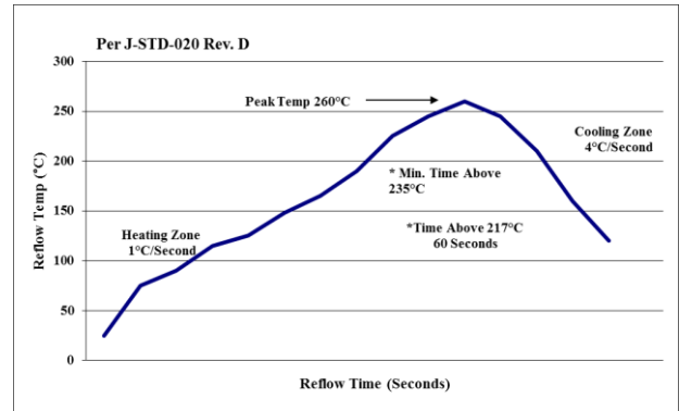
Figure 23. Recommended linear reflow profile using Sn/Ag/Cu solder.
