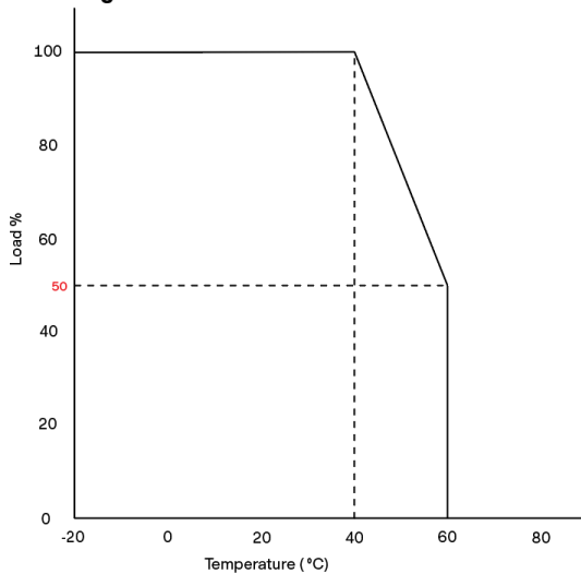
Derating curve
