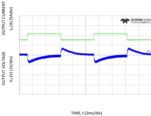
Figure 13. Transient Response to Dynamic Load Change from 50% to 100% at 48Vin, C_{out} = 330\mu F electrolytic + 15 x 2.2µF ceramic.
