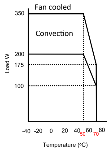
Power Derating Curve Others
