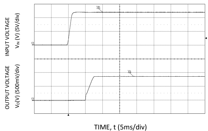
Figure 18. Typical Start-up Using Input Voltage (VIN = 12V, Cext=22µF, Io = Io,max).
