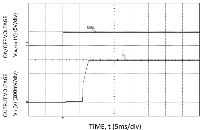
Figure 5. Typical Start-up Using On/Off Voltage (Io = Io,max, Vin=12V,Cext= 22µF).
