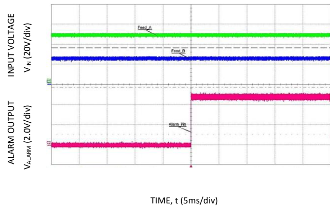
Fig 13: ALARM Output change of state with input voltage dropout
