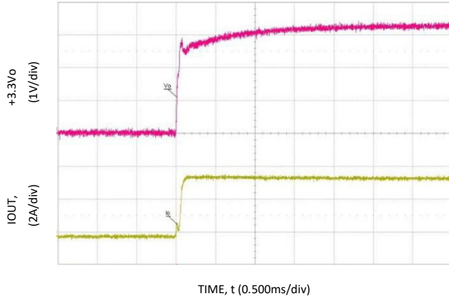
Fig 10: 3.3V Turn-On
