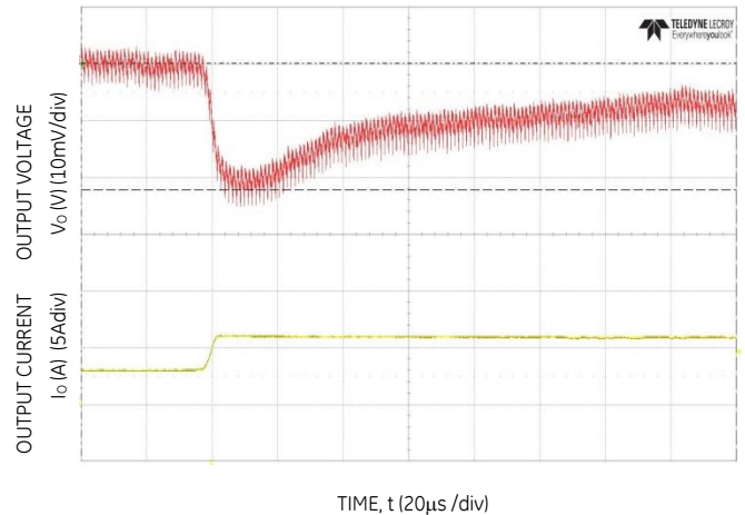
Figure 10. Transient Response to Dynamic Load Change from 50% to 100% at 12Vin, C out =3x47μF+2x330μF, C Tune =5600pF, R Tune =300Ω
