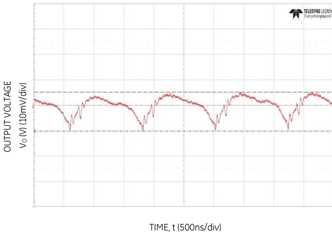
Figure 9. Typical output ripple ( C_o=2 \times 47 \mu F ceramic, V_{IN} = 12V , I_o = I_{o,max} , 20MHz BW).
