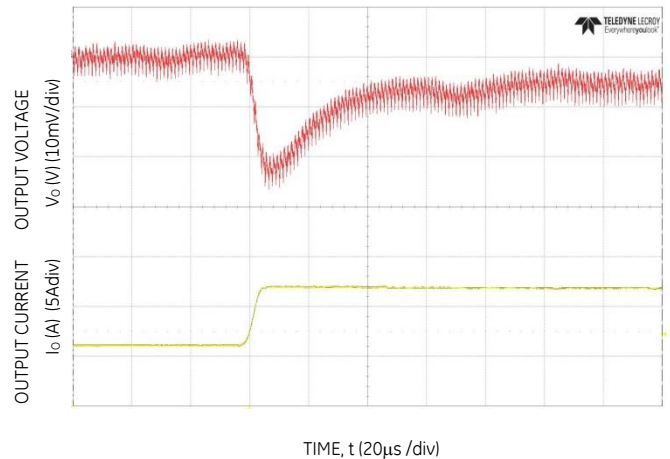
Figure 10. Transient Response to Dynamic Load Change from 50% to 100% at 12Vin, C_{out}=4 \times 47 \mu F + 3 \times 330 \mu F , C_{Tune}=10nF , R_{Tune}=300
