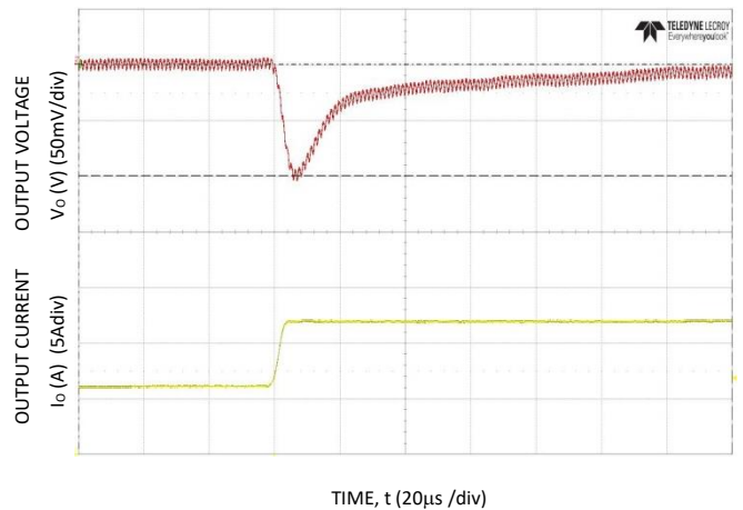
Figure 34. Transient Response to Dynamic Load Change from 50% to 100% at 12Vin, Cout=6x47uF, CTune=1200pF, RTune=300
