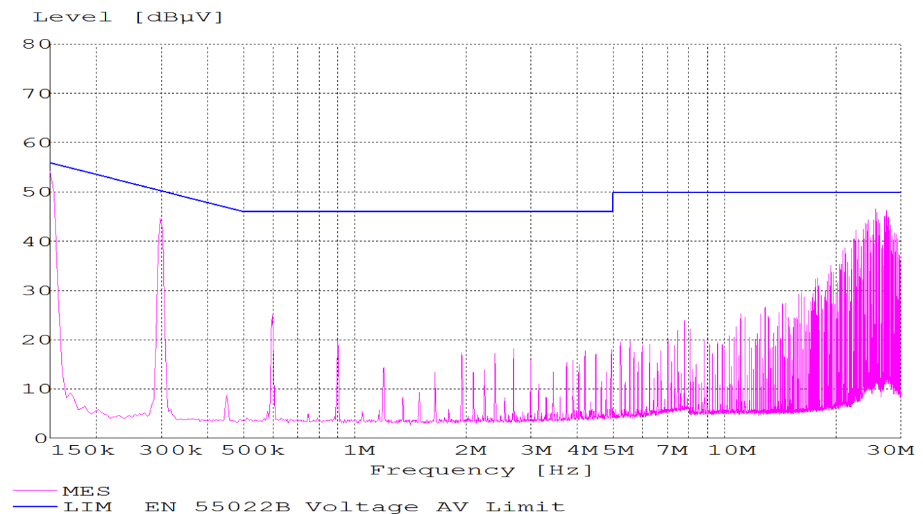
Figure 25. EMC Considerations
