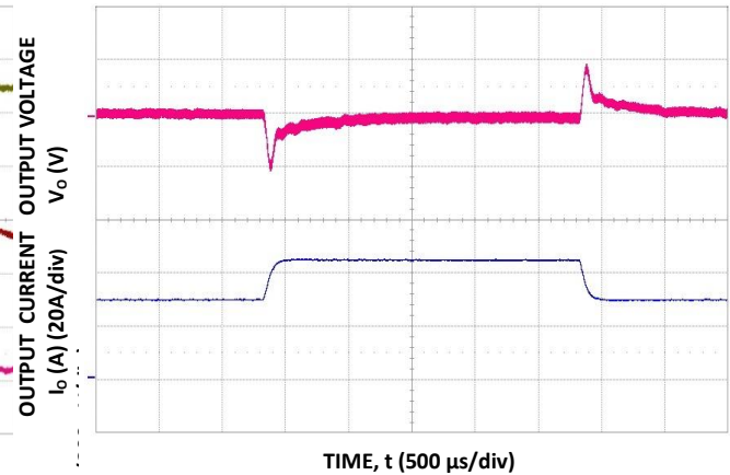
Figure 4. Typical Transient Response to 1A/μs Step Change in Load from 50% to 75% to 50% of Full Load, C_o = 2400\mu F and 48 V dc Input.
