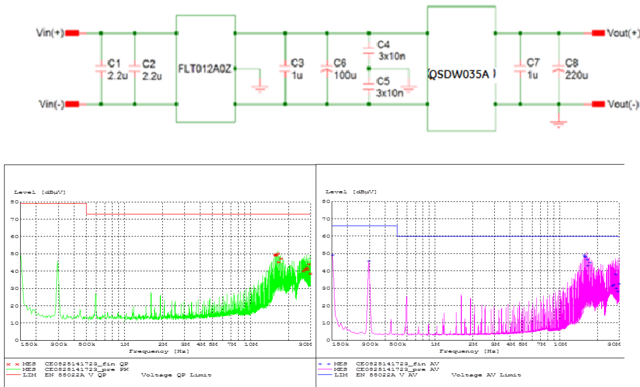
Figure 25. EMC Consideration
