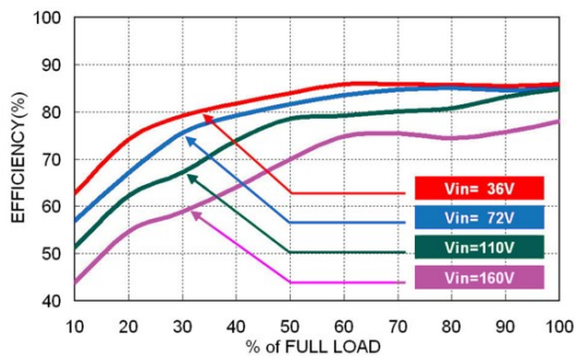
Efficiency Versus Output Load
