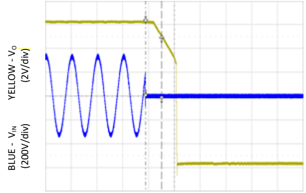
Time, t (20mSec/div)
