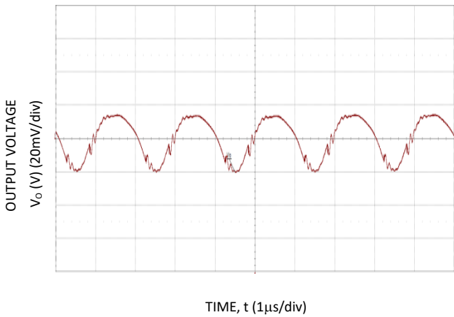
Figure 27. Typical output ripple and noise ( C_o=7x22\mu F ceramic, V_{in} = 12V , I_o = I_{o,max} ).
