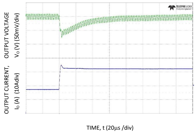
Figure 28. Transient Response to Dynamic Load Change from 50% to 100% at 12Vin, C_{out}=8x47\mu F+2x330\mu F , C_{Tune}=2700pF , R_{Tune}=221\Omega
