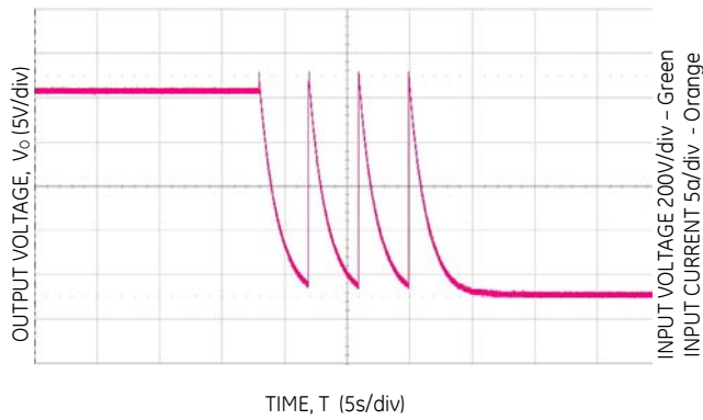
Figure 3. Overtolerance shutdown
