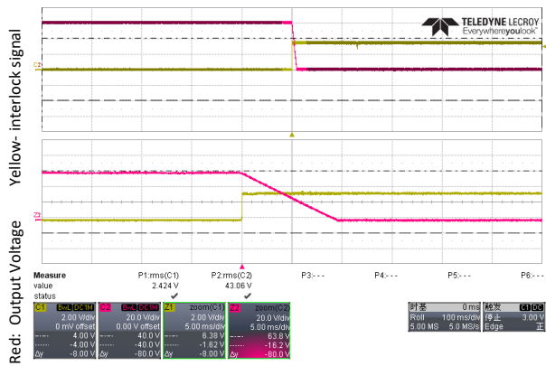
Figure 19: Time delay from interlock reverse and output shut down. interlock signal can be used as quick turn off signal.
