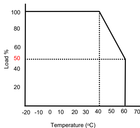
Derating curve
