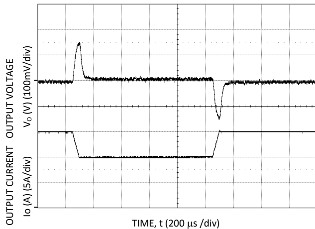
Figure 9. Transient Response to Dynamic Load Change, 0.1A/µS, from 75% to 50% to 75% of full load.
