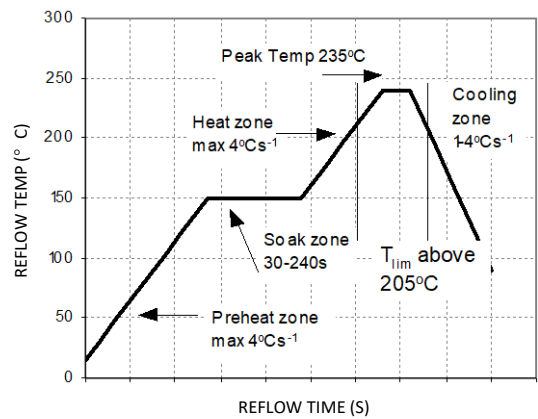
Figure 23. Reflow Profile for Tin/Lead (Sn/Pb) process
