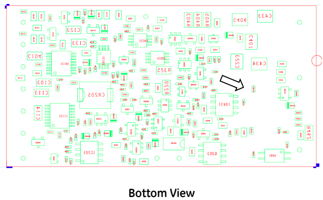
Figure 16. Location of Over Temperature Protection thermal sensors, T_{OTP} (Trip Point = 125^{\circ}C \pm 5^{\circ}C )
