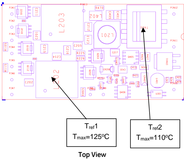
Figure 15. Thermal Reference Point, T_{ref} locations
