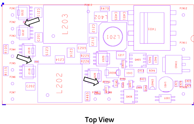
Figure 16. Location of Over Temperature Protection thermal sensors, T_{OTP} (Trip Point = 125^{\circ}C \pm 5^{\circ}C )
