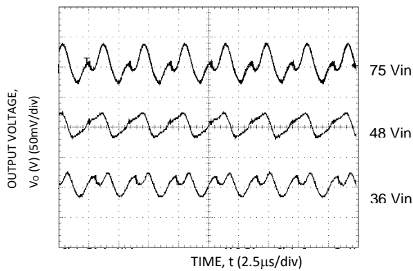
Figure 9. Typical Output Ripple and Noise at Room Temperature and I_o = I_{o, max} .
